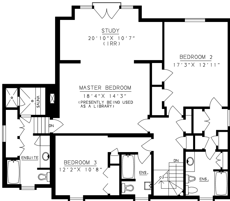
SECOND FLOOR 1,573 SQ.FT.
