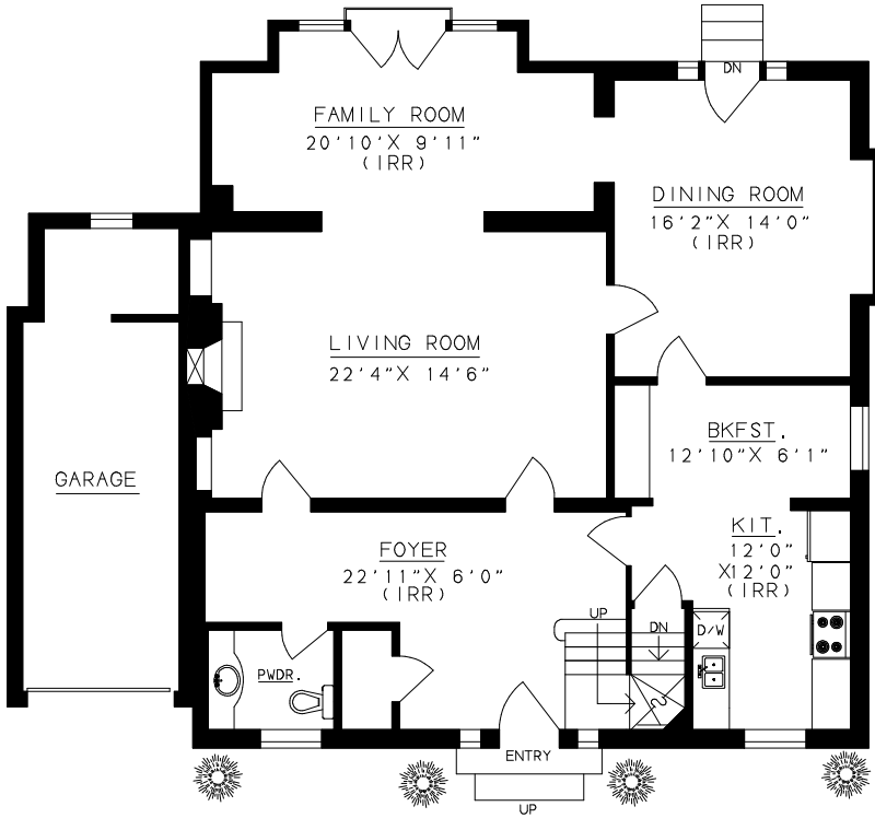
FIRST FLOOR 1,427 SQ.FT.
